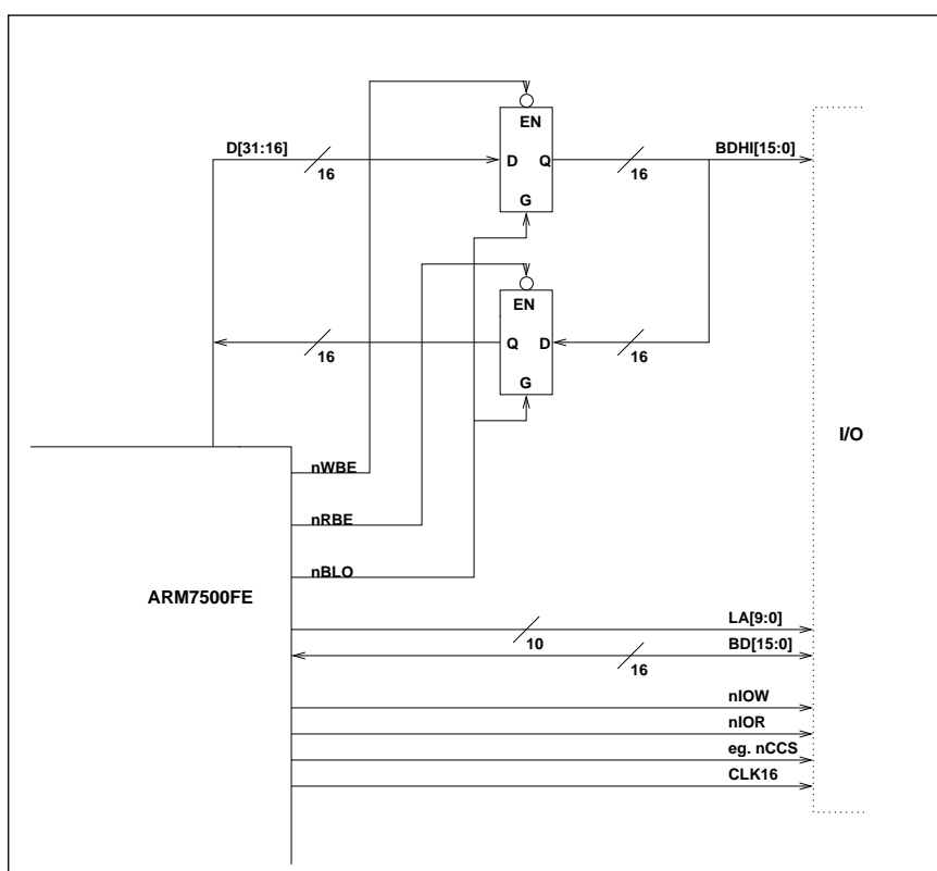
Figure D-1: 32-bit I/O interface
