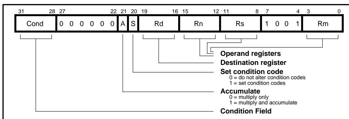
Figure 5-13: Multiply instructions
