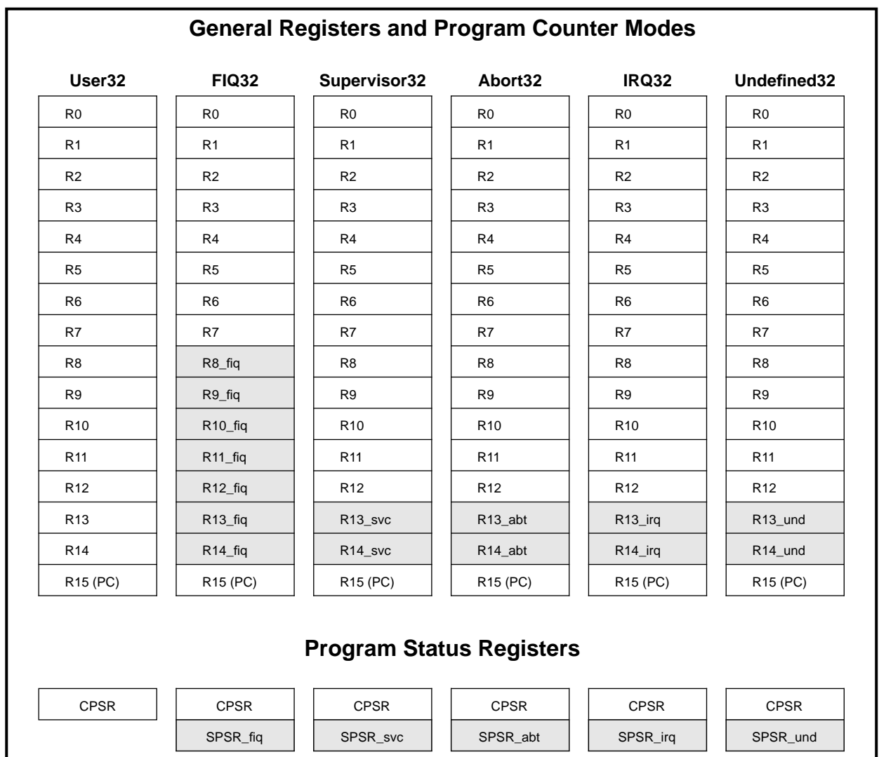
Figure 4-3: Register organization
