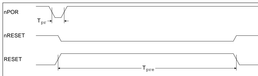
Figure 19-1: nPOR timing diagram
