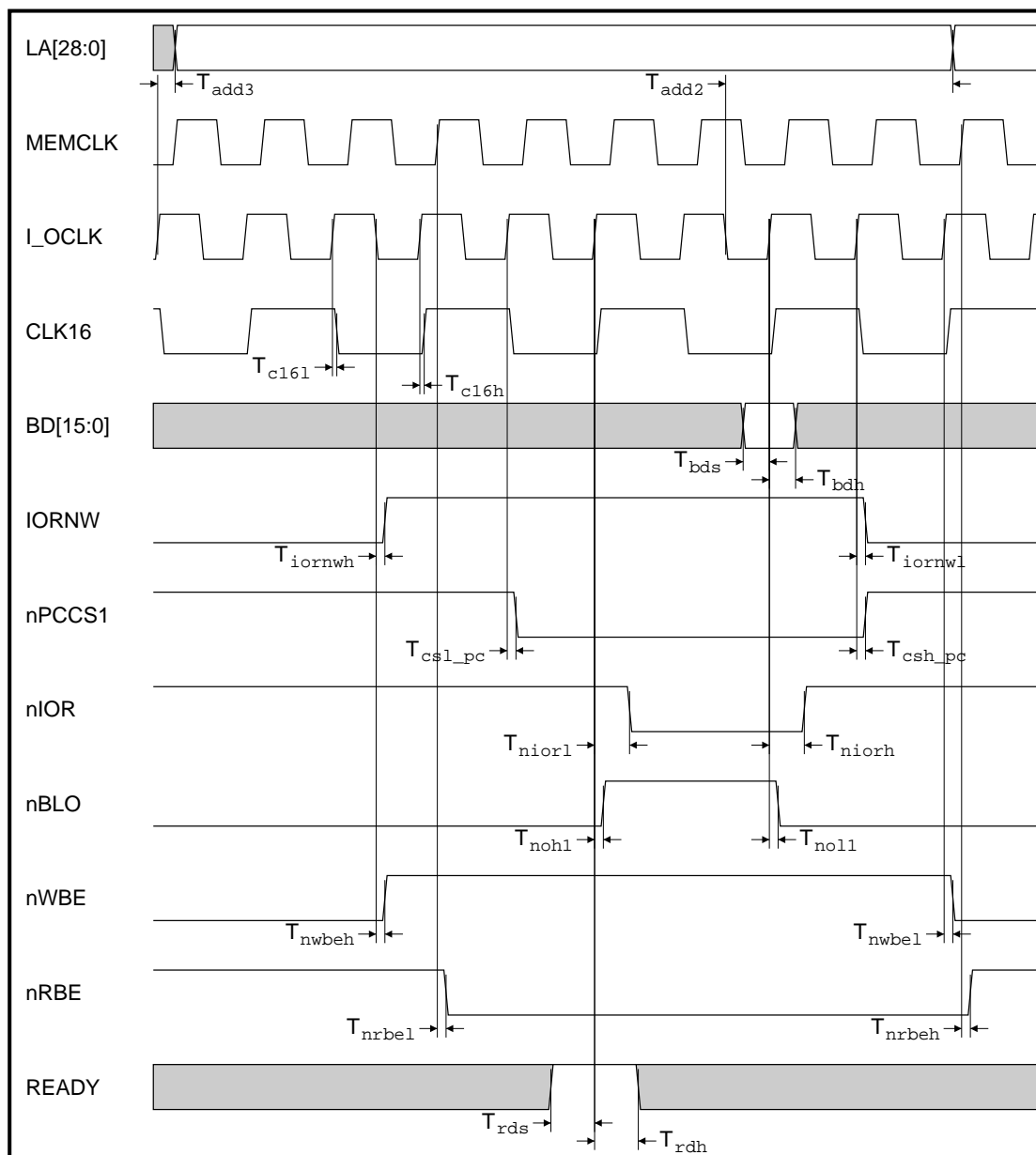
Figure 18-12: 16 MHz Type D read I/O cycle
