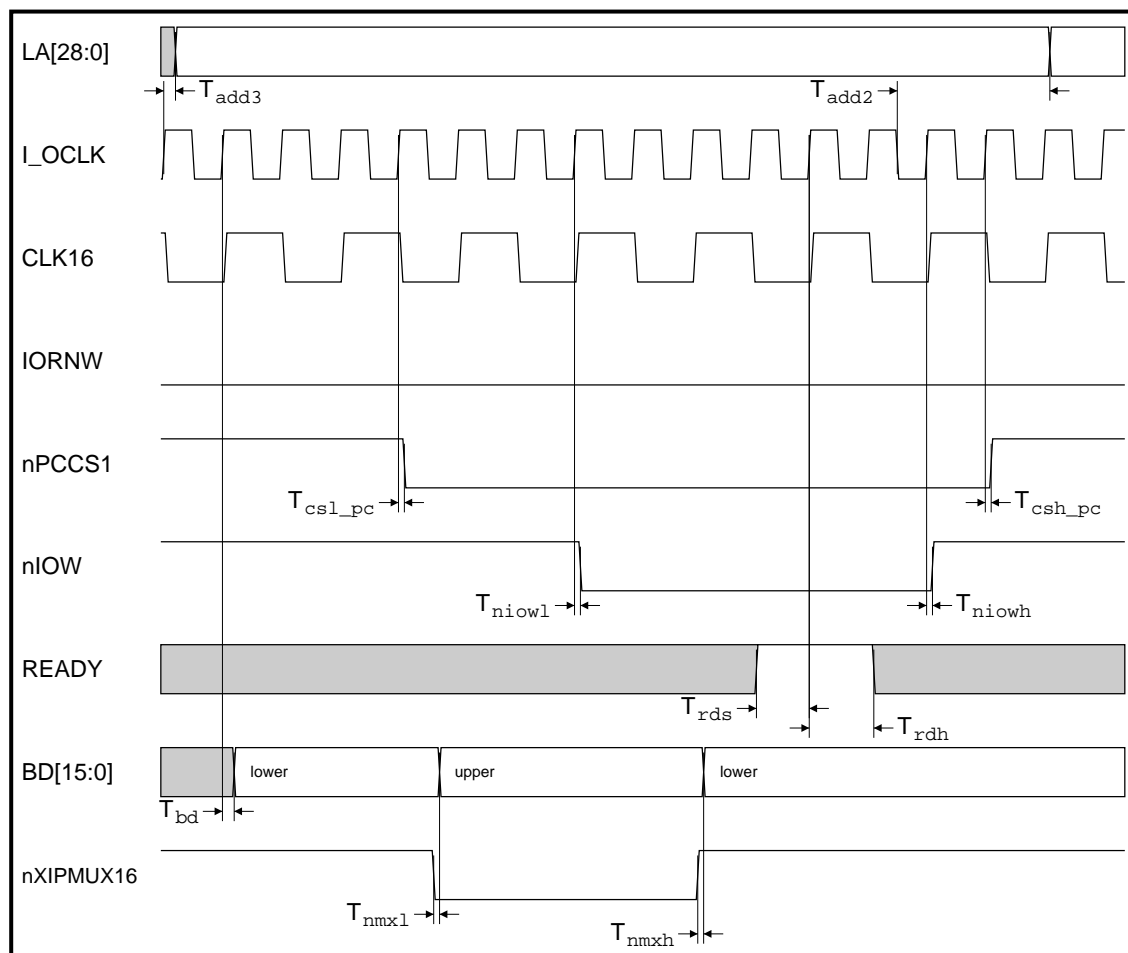
Figure 18-20: 16 MHz Type B write I/O cycle with PCMCIA
