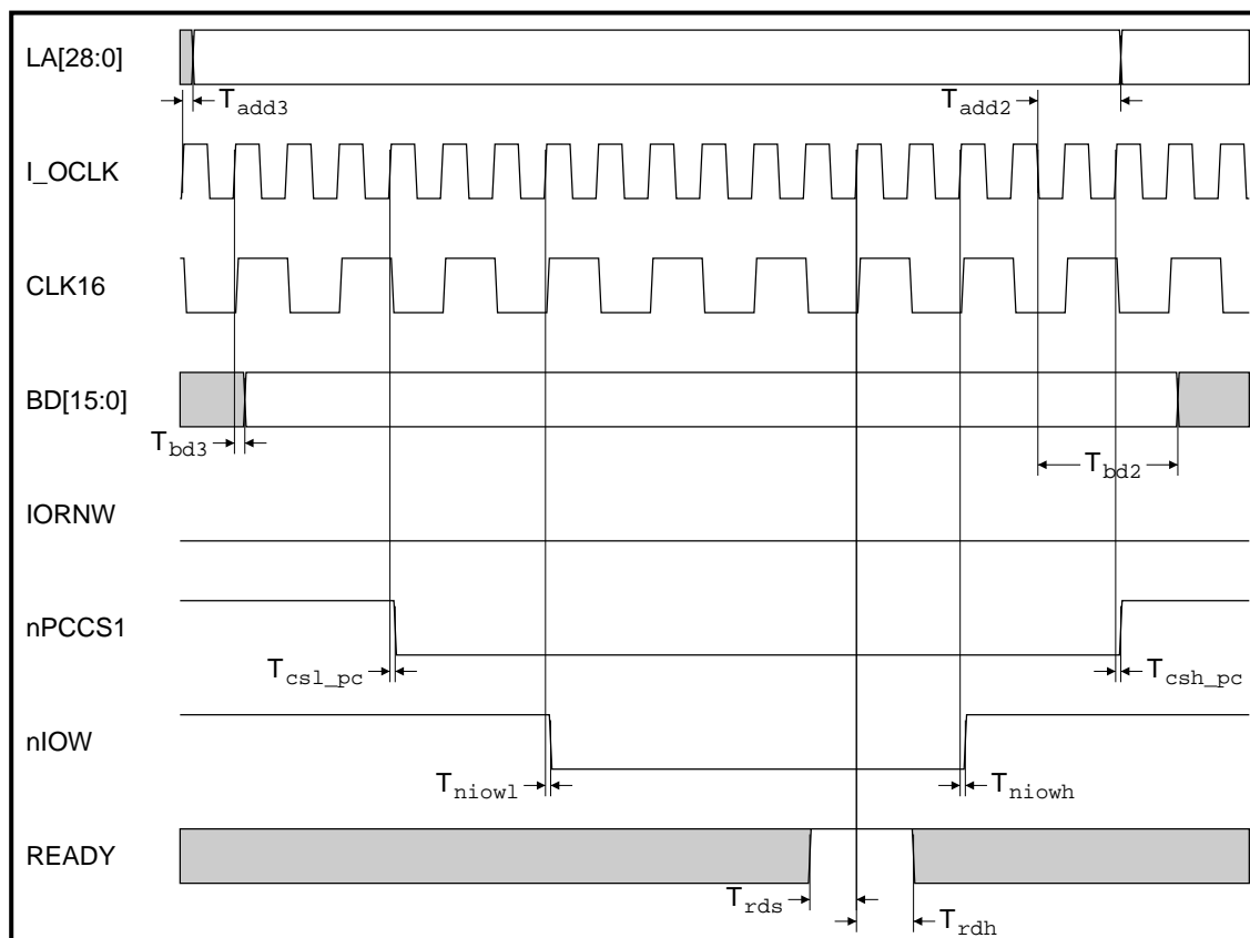
Figure 18-18: 16 MHz Type A write I/O cycle
